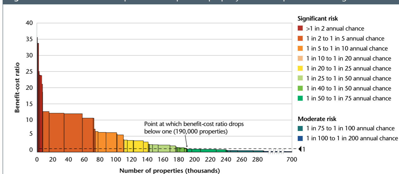
Figure 2.6: Cost curve to show potential for uptake of property-level flood protection in England
