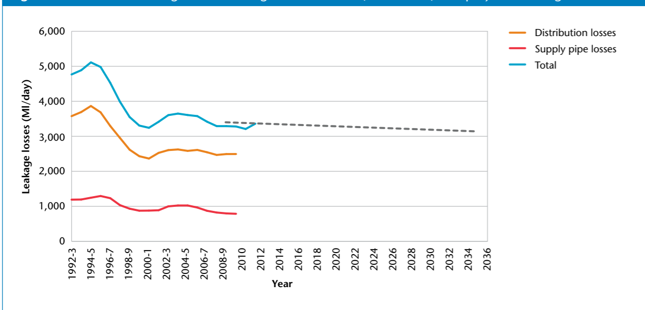
Figure 3.8: Measured leakage losses for England and Wales (1992-2011) and projected leakage out to 2035
