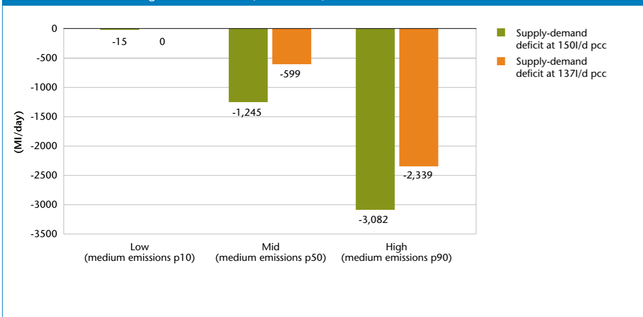
Figure 3.5: The effects on supply-demand deficit of a reduction in per capita consumption (pcc) from 150l/d to 137l/d for England and Wales (2010-2039)
